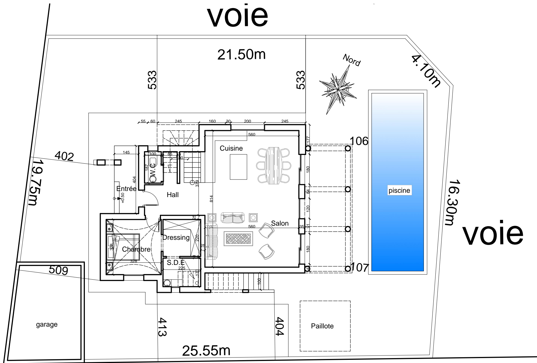
Plan RDC sc: 129.70m 2
